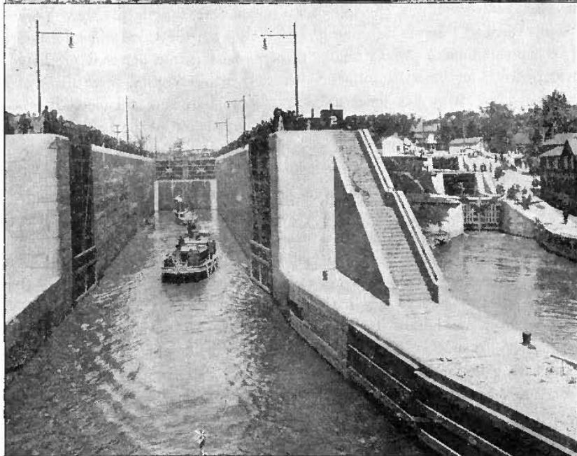
Above: First canal lock in New York State built at Little Falls (1796); length 70 ft., width 10 ft.
